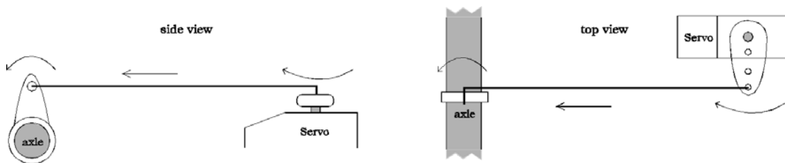
Figure 9. The tilting axle, controlled by a servo.
