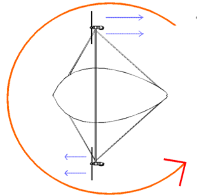
Figure 4. Horizontal steering.
